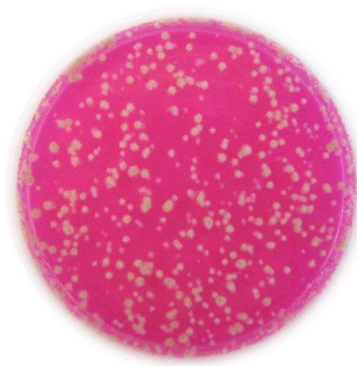
DRBC Agar (Dichloran Rose Bengal Chloramphenicol) Brown colonies and reduced size
