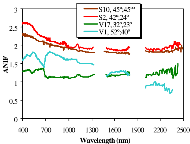
Fig. 8. Wavelength dependence of Anisotropy factor. The legend informs us about the sample name, the view zenith angle and the SZAs.
