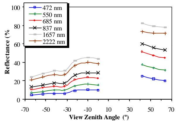
Fig. 6. Bidirectional Reflectance Factor at different view zenith angle in the principal plane. SZA=24^\circ
