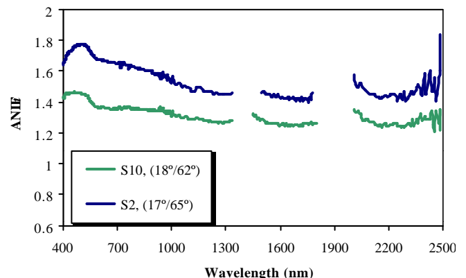
Fig 9. Anisotropy factor due to the illumination angle. Legend indicates field. and SZAs involves in the calculation.
