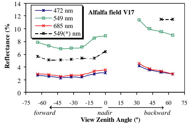
Fig. 4. BRF vs. view zenith angle in the principal plane for the alfalfa V17 canopy, SZ=23° and for the wheat V1 canopy only at 549(*) nm, SZ=40°
