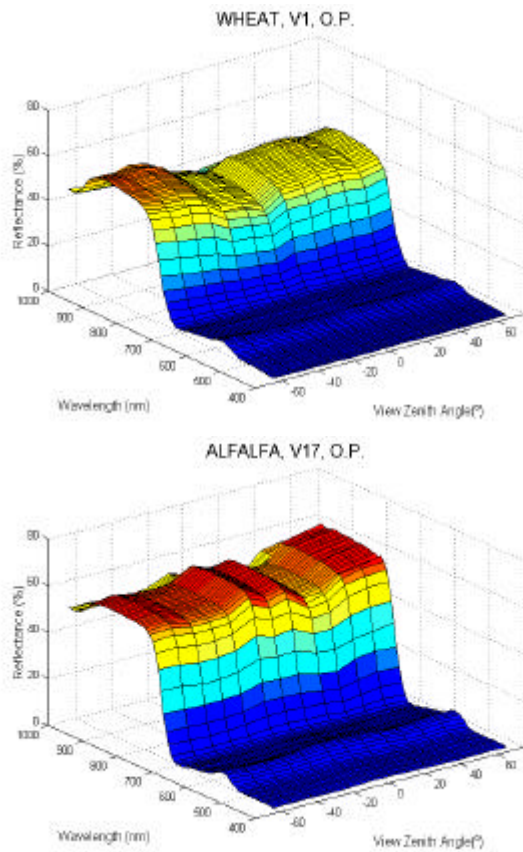
Fig. 3. Bidirectional Reflectance Factor vs. View Zenith Angle in the Orthogonal Plane: a) Wheat (V1), SZ=34°, b) Alfalfa (V17), SZ=19°
