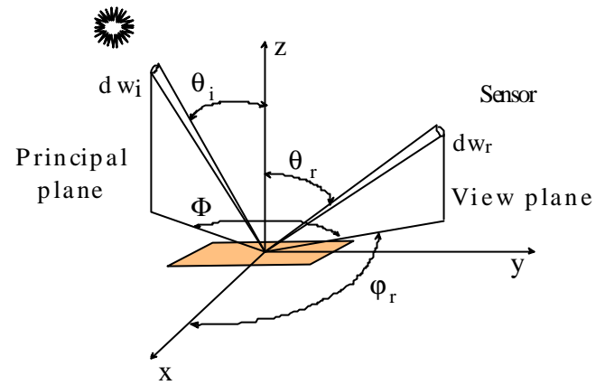
Fig1. Coordinate system defining geometry of incident and reflected elementary beams: d\omega (solid angle element), \mathbf{q} (zenith angle), \mathbf{j} (azimuth angle), i (illumination direction), r (viewing direction) and \Phi (azimuth relative angle).
