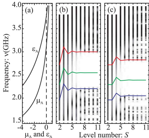
Fig. 1. (Color online) (a) Frequency behavior of the constitutive parameters corresponding to the MM layer. (b) Fibonacci and (c) Tribonacci photonic spectra at normal incidence for different generation levels.
