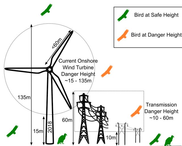
FIGURE 2 Danger height band definitions for energy infrastructure within which birds could be vulnerable to collision. The majority of transmission power lines (66 kV and over) range from 10 to 60 m in height (National Grid, 2014). For current onshore wind turbines, we derive a rotor swept zone ranging from 15 to 135 m above-ground (Pierrot, 2018; Thaxter et al., 2019)
