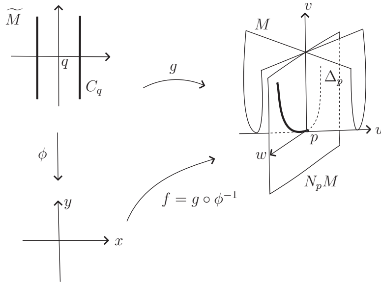
FIGURE 1. The Whitney umbrella surface of Example 1.3.
