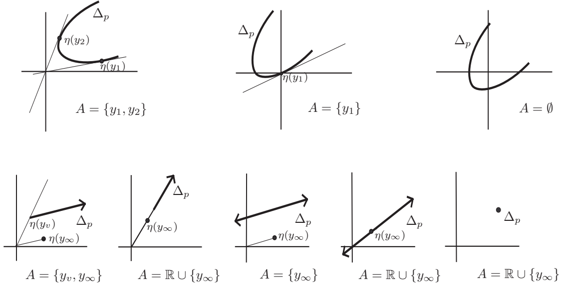
FIGURE 2. Possibilities for \Delta_p and the set A of asymptotic directions of M at p .
