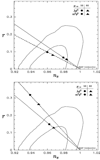
FIG. 1. Plot of r versus n_s . The contours show the 68% and 95% C.L. derived from WMAP5 (in combination with baryon acoustic oscillations BAO + SN) [3]. We consider V(\phi) = m^2 \phi^2 (solid line) and V(\phi) = \lambda \phi^4 (dashed line). The symbols show the prediction from each of this models in terms of the number N of e -folds. The top part corresponds to the prediction of our formulas, while the bottom one corresponds to the standard prediction.
