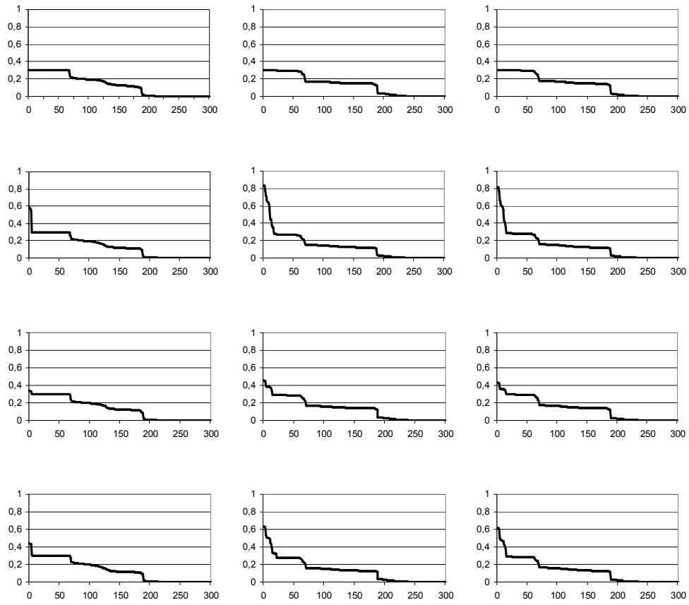
Figure 2. Observed exposure for different settings of the multiple objective exposure control method r_{\max}=0.30
