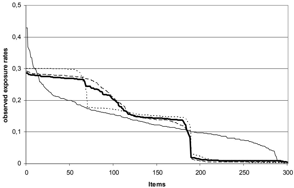
Figure 3. Observed exposure rates for multiple objectives (dotted), Sympton-Hetter (dashed), Alpha-stratified (thin), and Progressive (thick) exposure control.
