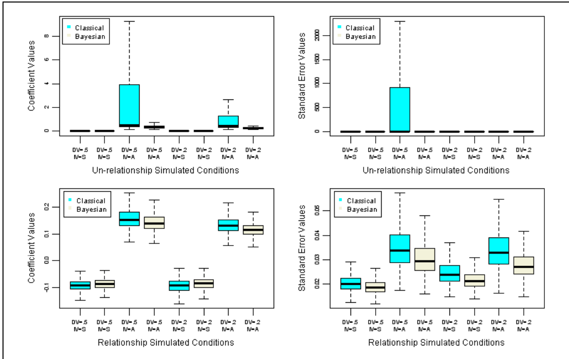
Figure 2. Coefficient Estimates and Standard Errors of the Continuous Independent Variable Based on Classical Estimation and Bayesian Estimation. Unrelated and Related Conditions in a Logistic Regression Model.
