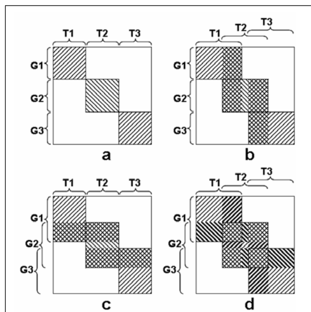
Figure 1: Four standard calibration designs oriented to link the parameters of the IB items on a common scale.
