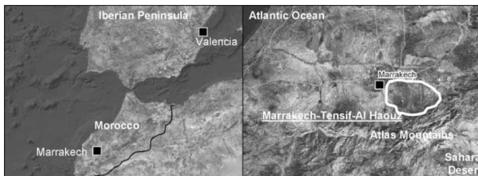
Figure 1. Location of the study area (delimited with a white line) in the Oued Tensif water catchment ( 31.658^{\circ}\text{N} , 7.608^{\circ}\text{W} , 586 m asl) in Marrakech (Morocco) and the reference station at Burjassot ( 39.508^{\circ}\text{N} , 0.418^{\circ}\text{E} , 60 m asl) in Valencia (Spain).
