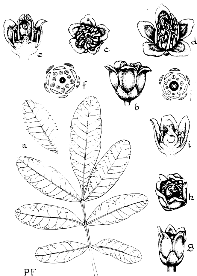
Figure 2 Schinus terebinthifolius , leaf and flowers. a. Leaf outline; toothed leaflet above; b-f. male flower, b. from the side, c. from above, early stage, d. from above, late stage, e. in longitudinal section, f. floral diagram; g-i. female flower, g. from the side, h. from above, i. in longitudinal section; j. floral diagram. (Tomlinson, 1980)
