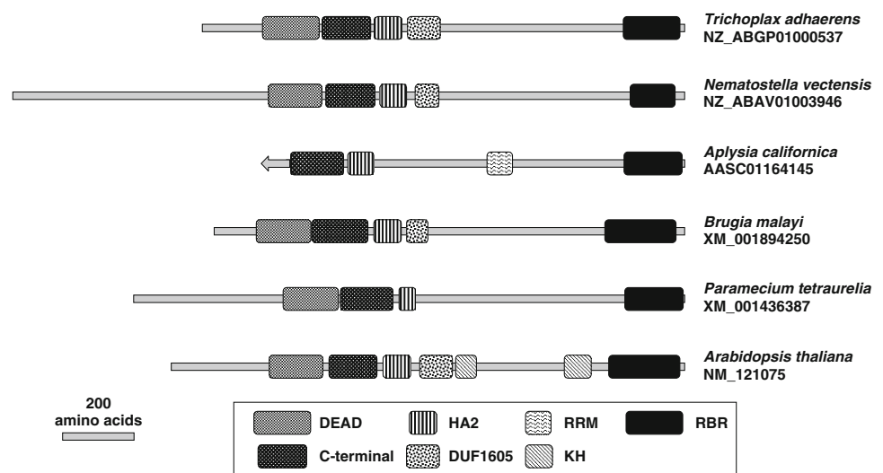
Fig. 2 Structures of helicase-containing RBR proteins. The arrow in the Aplysia sequence indicates that it has not been possible to establish its N-terminal end
