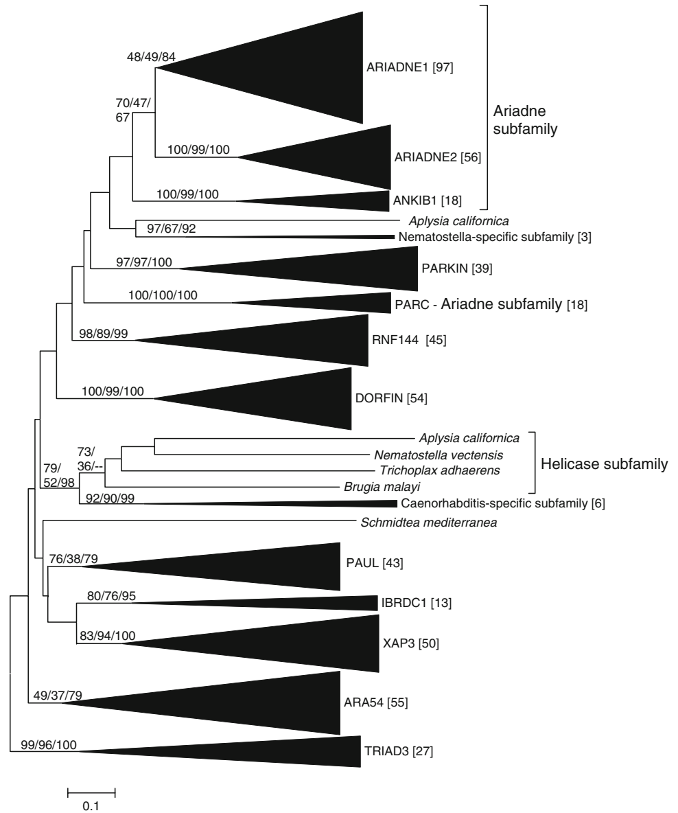
Fig. 1 Phylogenetic tree of RBR sequences. Names refer to both genes (orthology groups) and subfamilies, except for the Ariadne subfamily, which can be divided into four orthology groups (Ariadne1, Ariadne2, ANKIB1, PARC), as indicated. Numbers in brackets refer to the number of sequences in each branch. Bootstrap values, in percentages, are shown above the lines, ordered as follows: NJ/MP/ML. MP values tend to be lower than the rest because the MP analyses were not very exhaustive given the large amount of sequences, what makes difficult to detect the optimal trees (see “Methods” section). Dashes indicate that a particular branch was not supported by the ML analysis. A full account of this tree, including all species names and accession numbers, can be found in Supplementary Files 1 and 2
