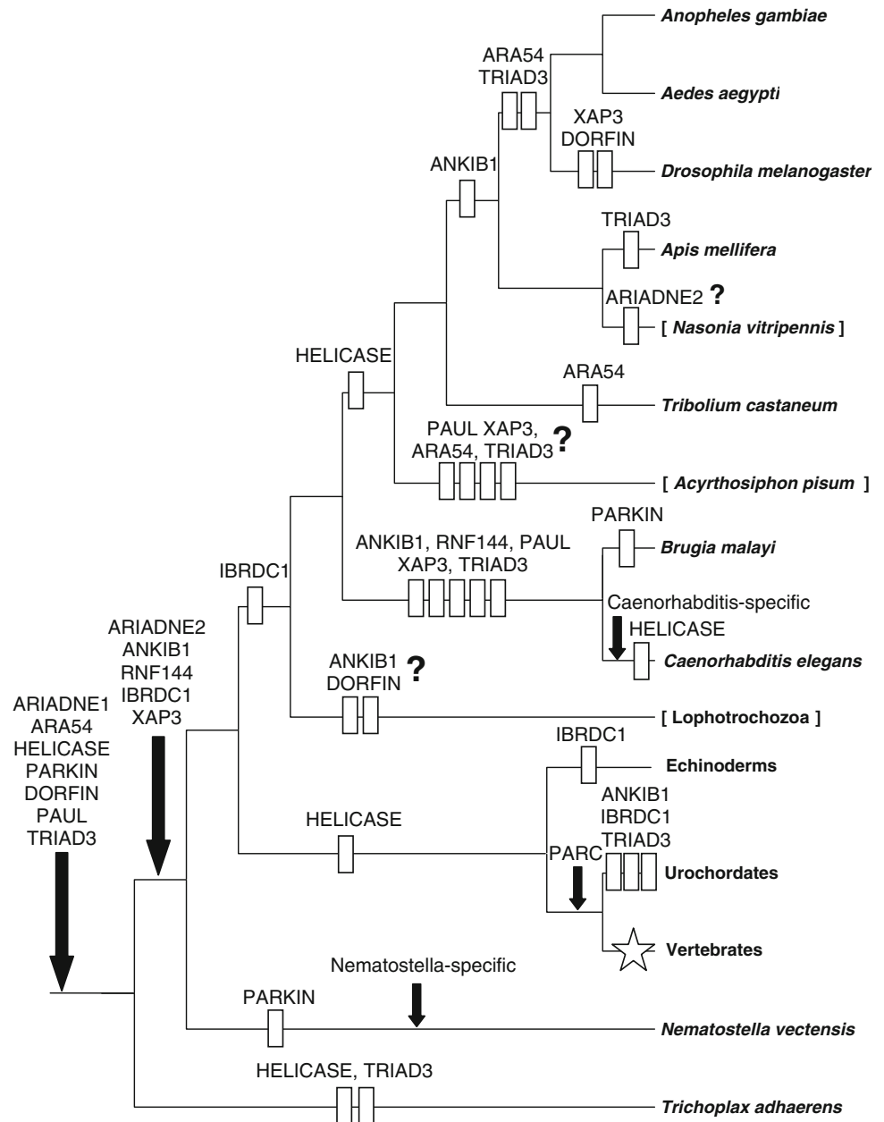
Fig. 3 Diversification and simplification of the RBR family. The simplest hypothesis that explains all available data is summarized. I have assumed a basal phylogenetic position for placozoans, as described by Srivastava et al. (2008), and, for protostomes, the ecdysozoa/lophotrochozoa split. Arrows indicate appearances and rectangles indicate losses. The star indicates multiple appearances and losses associated to the genome duplications in vertebrates. Question marks have been added to indicate that results for branches for which there is no complete genomic data (in which the names are indicated in brackets) are still provisional
