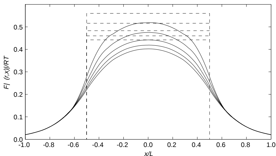
Fig. 5. Distribution of the electric potential for a pore of length L = 5/\bar{j} and radius a = 1.0/\bar{j} (each curve corresponds to values of r/a : 1.0, 0.8, 0.6, 0.4, 0.0 from top to bottom). The rest of the parameters are the same as in Fig. 2. Curves corresponding to the discontinuous approach (dashed lines) are also shown for comparison.
