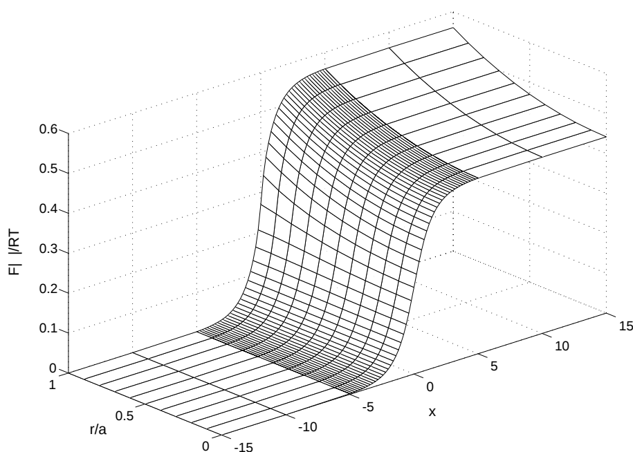
Fig. 2. Electric potential distribution (in RT/F units) for a pore with X = 50 mM, j a = 1.0 , and a bulk electrolyte concentration c = X .
