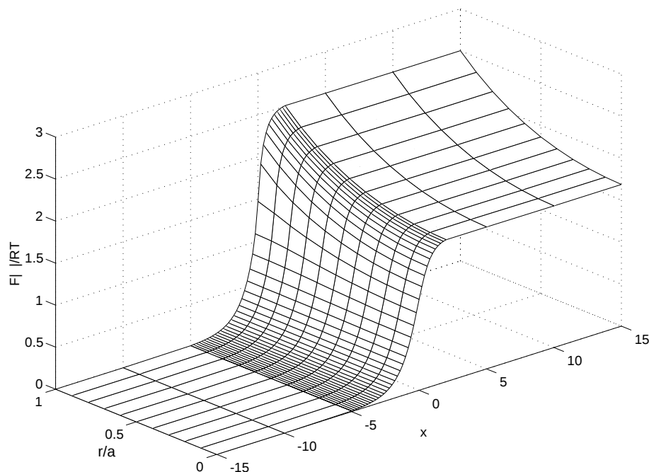
Fig. 3. Electric potential distribution (in RT/F units) for a pore with X = 0.4 M, j a = 1.0 , and a bulk electrolyte concentration c = X/8 = 50 mM. The solution has been obtained by solving Eq. (12) by means of a finite element method.
