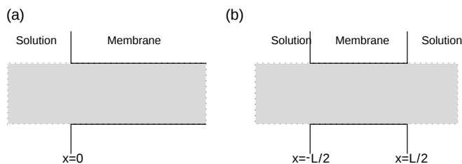
Fig. 1. Interfacial regions considered: (a) semi-infinite pore and external solution, (b) finite pore of length L and external solutions.
