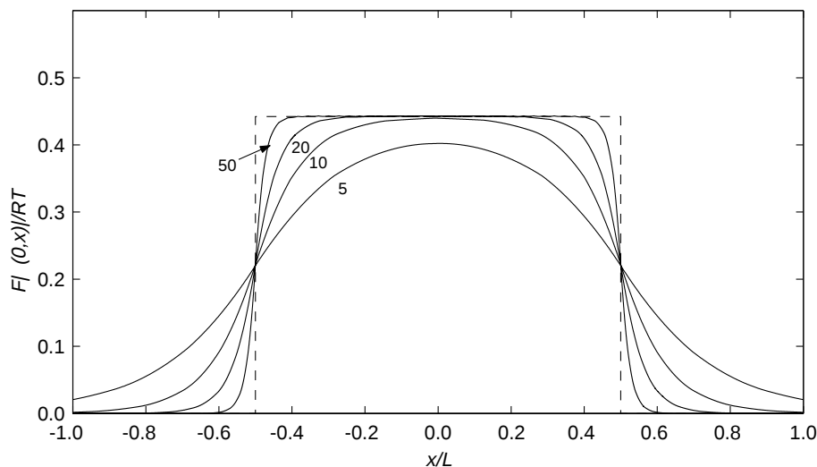
Fig. 4. Axial distribution of the electric potential across pores of different lengths (values of j L shown) and equal radii, j a = 1.0 . The rest of the parameters are the same as in Fig. 2. The curve corresponding to the discontinuous approach (dashed line) is also shown for comparison.
