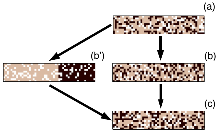
Fig. B.1. Two possible trajectories joining the disordered configurations (a) and (c) of two mixed fluids. The trajectory going through (b') is forbidden by the Maupertuis principle since it is possible to find disordered configurations (b) between (a) and (c) so that the abbreviated action ( \equiv the length of the trajectory between (a) and (c) in the 3N -dimensional configuration space) is a minimum.
