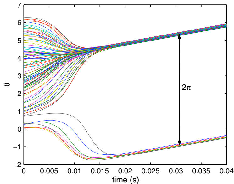
Fig. 1. Time evolution of the phases of 100 oscillators for strong coupling K = 5 obtained by numerical integration of Eq. (32). The system starts with a random distribution of phases and after a short transient all oscillators become synchronized with the emergence of two branches with the same effective frequency.
