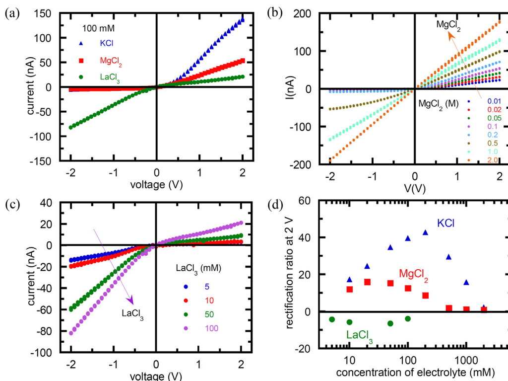
Fig. 2. (a) The I - V curves of KCl, MgCl 2 , and LaCl 3 . The reversal observed in the electrical rectification of the LaCl 3 curve suggests an inversion in the pore surface charge from negative to positive. (b) The I - V curves over a wide range of MgCl 2 concentrations demonstrate that this charge overcompensation does not occur. The arrow indicates the direction of increasing MgCl 2 concentration. (c) Charge reversal is observed for LaCl 3 concentrations higher than 5 mM. The arrow indicates the direction of increasing LaCl 3 concentration. (d) The electrical rectification ratios r = |I(+2 V)/I(-2 V)| > 1 for KCl and MgCl 2 and r = I(-2 V)/I(+2 V) < -1 for LaCl 3 as a function of the electrolyte concentration. The position of the maxima shifts with the cation charge number because of the different number of charges contributing to the pore conductance in each case.
