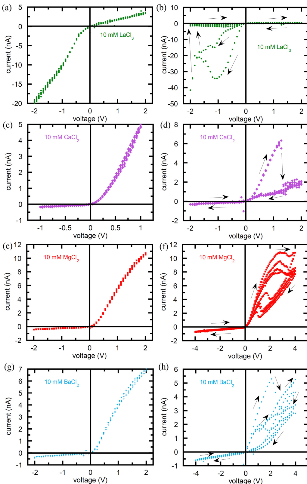
Fig. 7. (a) The I-V curve of \text{LaCl}_3 at 10 mM and voltages in the range [-2\text{ V}, +2\text{ V}] . (b) The I-V curve of \text{LaCl}_3 can also show a hysteretic behavior for these voltages if the pore has not been equilibrated previously in a \text{LaCl}_3 solution of concentration above 50 mM. (c) The I-V curve of \text{CaCl}_2 at 10 mM and voltages in the range [-1\text{ V}, +1\text{ V}] . (d) The I-V curve of \text{CaCl}_2 at high voltages in the range [-2\text{ V}, +2\text{ V}] shows a hysteretic behavior. (e) The I-V curves of \text{MgCl}_2 at 10 mM and voltages in the range [-2\text{ V}, +2\text{ V}] (f) The I-V curves of \text{MgCl}_2 at high voltages in the range [-4\text{ V}, +4\text{ V}] shows a hysteretic behavior. (g) The I-V curves of \text{BaCl}_2 at 10 mM and voltages in the range [-2\text{ V}, +2\text{ V}] . (h) The I-V curves of \text{BaCl}_2 at high voltages in the range [-4\text{ V}, +4\text{ V}] shows a hysteretic behavior. The arrows indicate the direction of the measurements with increasing time.
