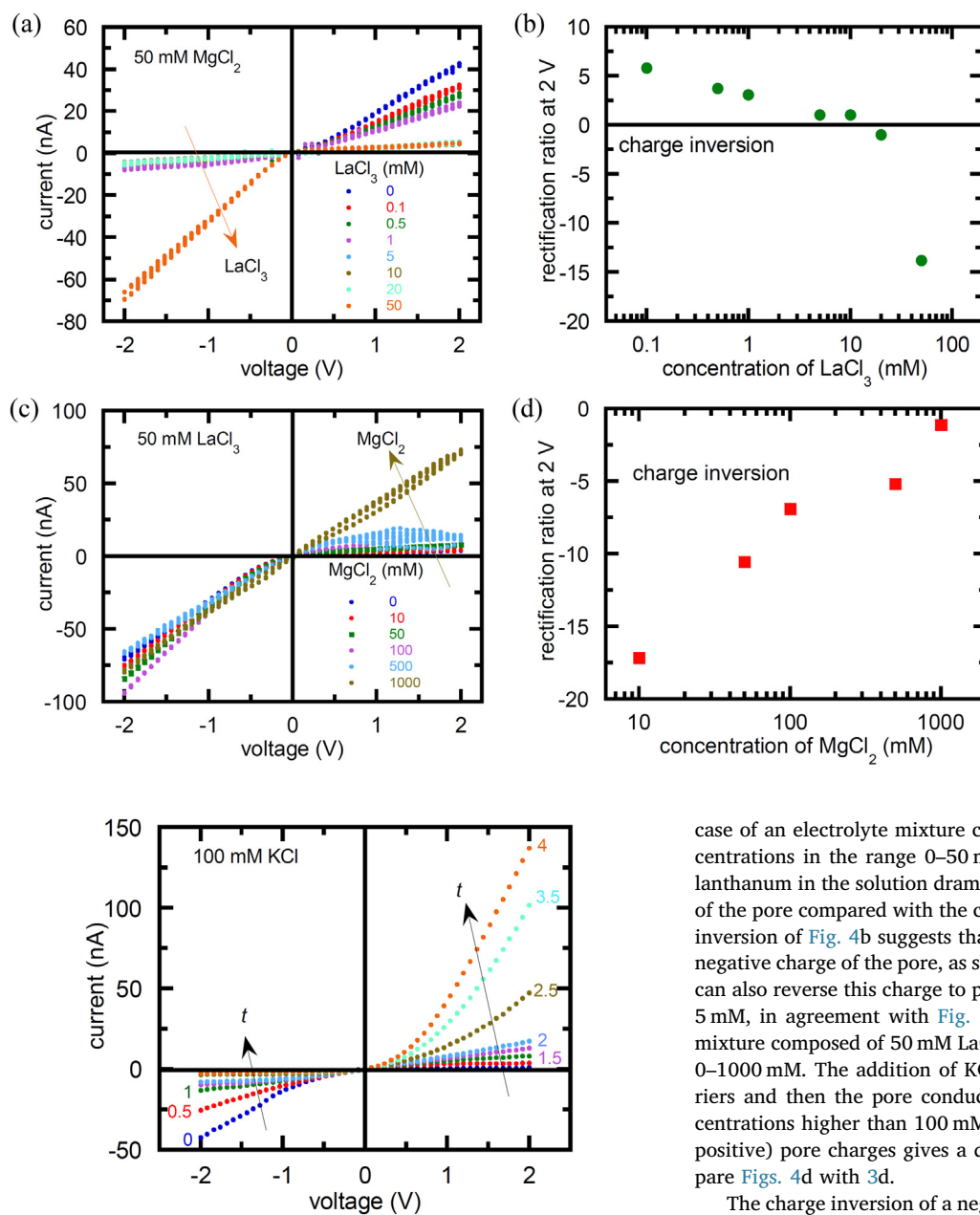
Fig. 6. The recovery of the I - V curve for a nanopore initially immersed in 50 mM LaCl_3 . At t = 0 h, the single-pore membrane is placed in the measuring cell, separating two 100 mM KCl solutions, under the constant action of an input 14 mHz triangular wave of amplitude 2 V. The current passing through the sample is then measured at the times (h) indicated close each curve.
