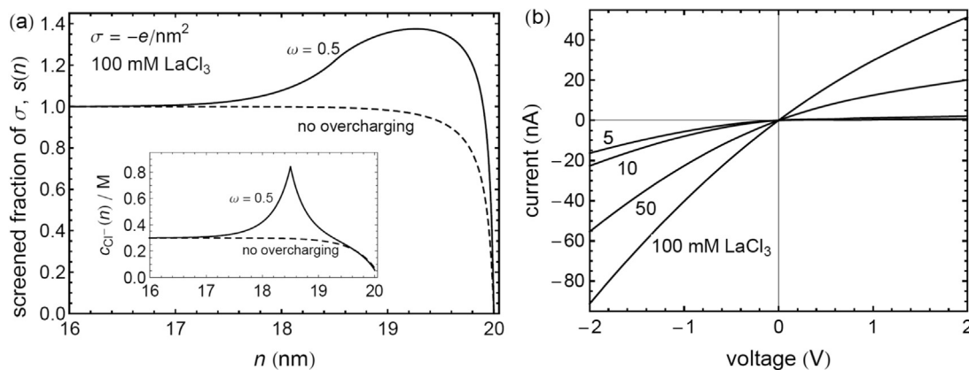
Fig. 9. (a) The fraction s(n) of the actual surface charge \sigma = -e/nm^2 that has been screened at position n = r\theta (normal to the pore surface and measured from its axis) can be larger than 100% due to the charge overcompensation by trivalent cations. A pore radius a = 20 nm has been considered here. The screening is close to 100% at a distance of a few Debye lengths, 1/\kappa_D , from the pore surface. The insets show the coion (chloride) concentration profile. The maximum shown at a distance d = 1.5 nm from the pore surface is in qualitative agreement with the results obtained previously by Monte Carlo simulations [10]. (b) The theoretical I-V curves calculated for a conical pore of geometrical characteristics L = 12.5 \mu\text{m} , a_R = 20 nm, a_L = 900 nm, and a_{\text{eff}}(x) = -\delta + a_L + (a_R - a_L)x/L , with an effective surface charge density \sigma_{\text{eff}} = +0.1 e/nm^2 , are in qualitative agreement with the experimental curves for \text{LaCl}_3 of Fig. 2c.
