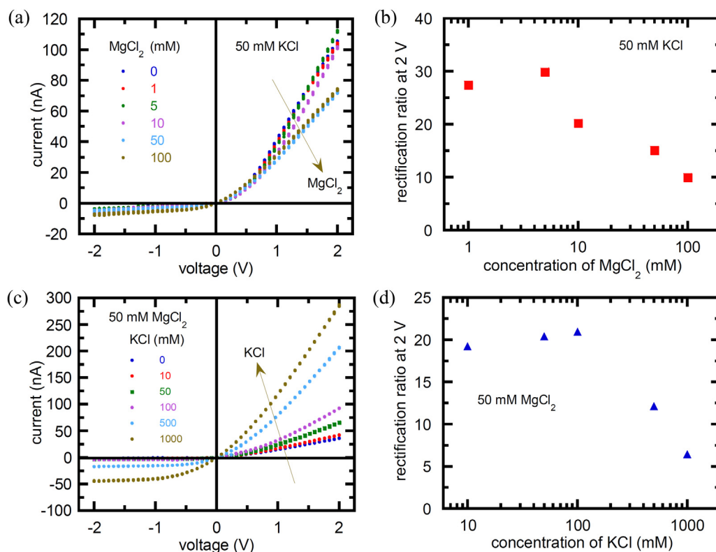
Fig. 3. (a) The I - V curves of mixtures of electrolytes at different concentrations. The KCl concentration is fixed to 50 mM and the MgCl_2 concentrations are changed between 0 and 100 mM. The arrow indicates the direction of increasing MgCl_2 concentration. (b) The corresponding rectification ratios. (c) The I - V curves obtained when the MgCl_2 is fixed to 50 mM and the KCl concentrations are increased from 0 to 1000 mM. The arrow indicates the direction of increasing KCl concentration. (d) The corresponding rectification ratios.
