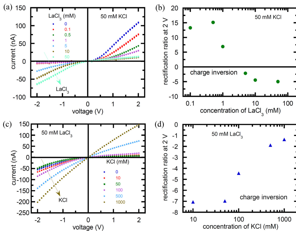
Fig. 4. (a) The I - V curves of mixtures of electrolytes at different concentrations. The KCl concentration is fixed to 50 mM and the LaCl_3 concentrations are changed between 0 and 50 mM. The arrow indicates the direction of increasing LaCl_3 concentration. (b) The corresponding rectification ratios. (c) The I - V curves obtained when the LaCl_3 concentration is fixed to 50 mM and the KCl concentrations are increased from 0 to 1000 mM. The arrow indicates the direction of increasing KCl concentration. (d) The corresponding rectification ratios.
