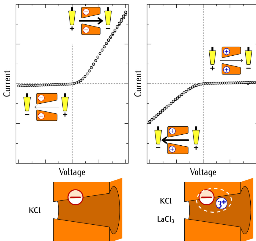
Fig. 1. Scheme of the charge reversal effect observed in the I – V curves of the nanopore due to the presence of \text{La}^{3+} in the external solutions.
