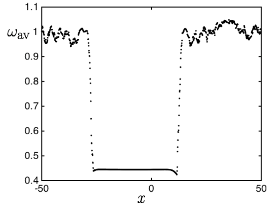
Fig. 3. Average frequency of the oscillators depending on their spatial position x for the chimera pattern of Fig. 2(c).
