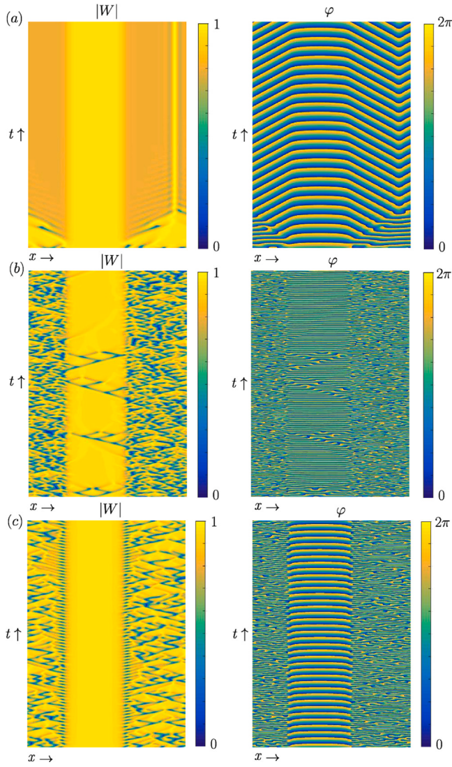
Fig. 2. Spatiotemporal evolution of the absolute value |W| (left panels) and the phase \varphi (right panels) of the complex order parameter W for a = 0.2, b = 0.5 (a); a = 0.75, b = 2.25 (b) and a = 0.75, b = 1.2 (c). Other parameter values are \mu = 1 and c_1 = 0.7 .
