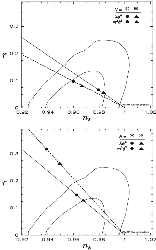
Fig. 1 Plot of r versus n_s . The contours show the 68 and 95% CL derived from WMAP5 (in combination with BAO + SN) [20]. We consider two representative inflation models: V(\phi) = m^2 \phi^2 (solid line), V(\phi) = \lambda \phi^4 (dashed line). The symbols show the prediction from each of this models in terms of the number N of e-folds of inflation for the monomial potentials. The top part corresponds to the prediction of our formulae, while the bottom one corresponds to the standard prediction
