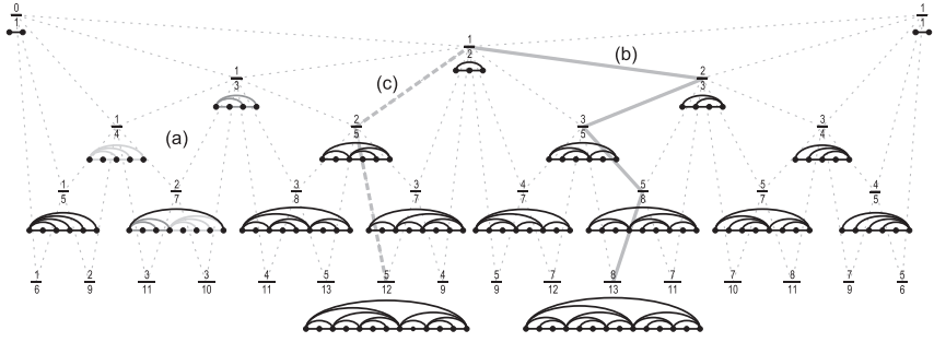
Figure 10 Six levels of the Farey tree and the periodic motifs of the graphs associated with the corresponding rational fractions p/q taken as dressed winding numbers \omega in the circle map (for space reasons only two of these are shown at the sixth level). (a) In order to show how graph concatenation works, we have highlighted an example using different grey tones on the left side: as 1/3 > 1/4 , G(1/3) is placed on the left, G(1/4) on the right and their extremes are connected to an additional link closing the motif G(2/7) . (b) Five steps in the Golden ratio route, b = 1 (thick solid line); (c) Three steps in the Silver ratio route, b = 2 (thick dashed line).
