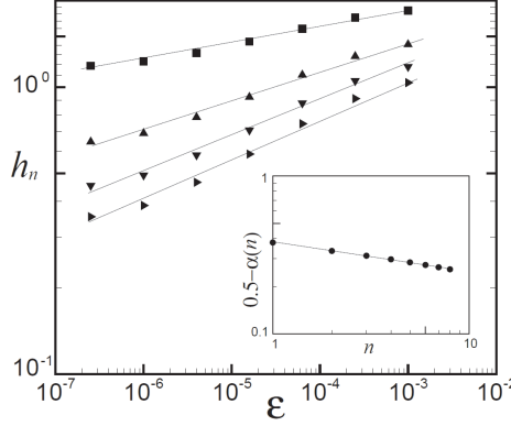
Figure 8 Log-log plot of the block entropies h_n constructed from degree distributions of n -sequence of connectivities in the HV graphs as a function of \epsilon : n = 1 (squares), n = 2 (up-triangles), n = 3 (down-triangles), n = 4 (right-triangles). A scaling of the form h_n \sim \epsilon^{\alpha(n)} is found. (Inset panel) Log-log plot of the convergence of \alpha(n) to the exponent associated to the Lyapunov exponent, as a function of n . A relation of the form [0.5 - \alpha(n)] \sim n^{-0.19} is found.
