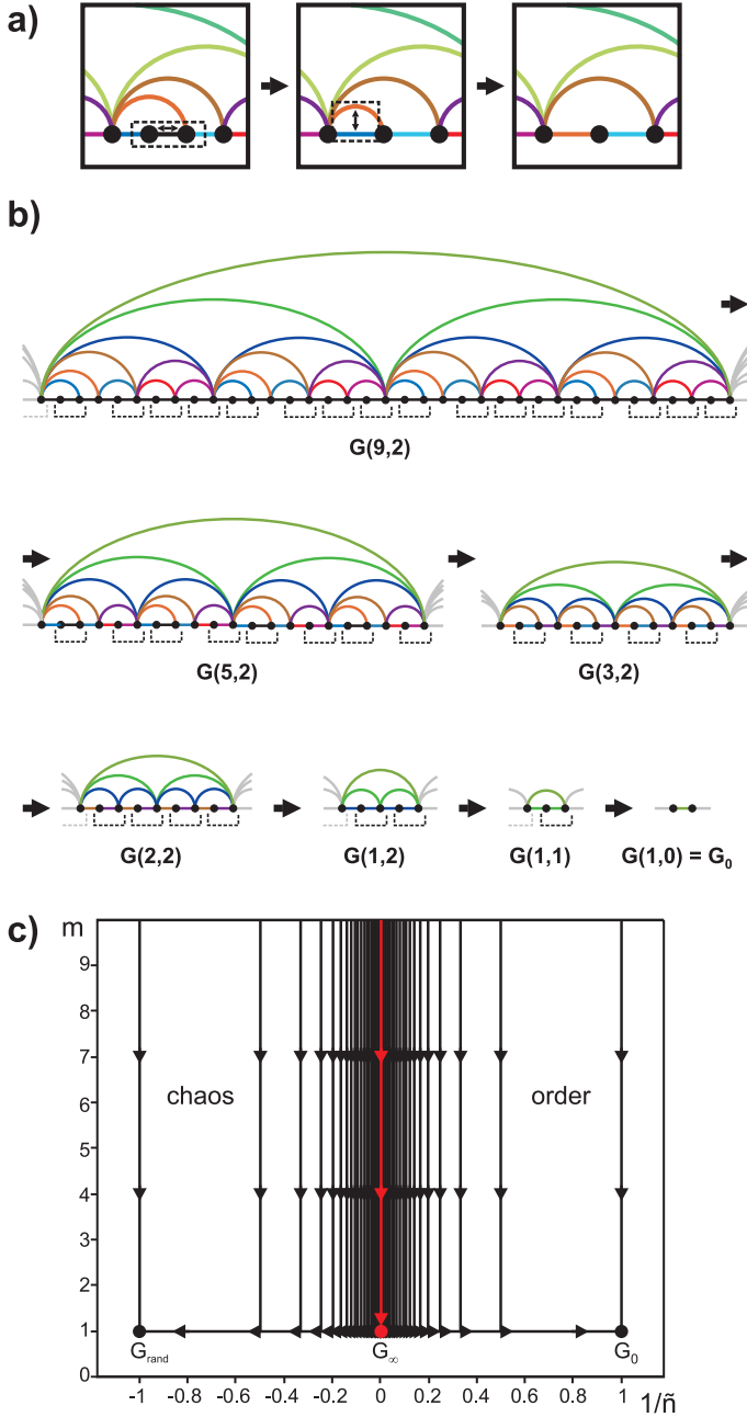
Figure 11 Renormalization process and network RG flow structure. (a) Illustration of the renormalization process: a node with degree is coarse-grained with one of its neighbors (indistinctively) into a block node that inherits the links of both nodes. This process coarse-grains every node with degree present at each renormalization step. (b) Example of an iterated renormalization process in a sample Feigenbaum graph at a periodic window with initial period after period-doubling bifurcations (an orbit of period ). (c) RG flow diagram.
