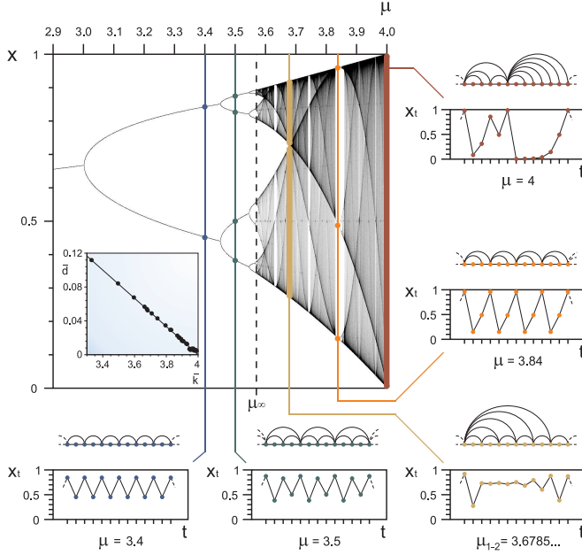
Figure 3 Feigenbaum graphs from the Logistic map x_{t+1} = f(x_t) = \mu x_t(1 - x_t) . The main figure portrays the family of attractors of the Logistic map and indicates a transition from periodic to chaotic behavior at \mu_\infty = 3.569946\dots through period-doubling bifurcations. For \mu \geq \mu_\infty the figure shows merging of chaotic-band attractors where aperiodic behavior appears interrupted by windows that, when entered from their left-hand side, display periodic motion of period T = m \cdot 2^0 with m > 1 (for \mu < \mu_\infty , m = 1 ) that subsequently develops into m period-doubling cascades with new accumulation points \mu_\infty(m) .
