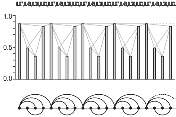
Figure 1 Illustrative example of the Natural Visibility algorithm. In the upper part we plot a periodic time series and in the bottom part we represent the graph generated through the Natural Visibility algorithm. Each datum in the series corresponds to a node in the graph, such that two nodes are connected if their corresponding data heights fulfill the visibility criterion of equation 1. Note that the degree distribution of the visibility graph is composed by a finite number of peaks, much in the vein of the Discrete Fourier Transform of a periodic signal. We can thus interpret the Visibility Algorithm as a geometric transform.
