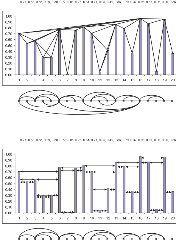
Figure 2 Illustrative example of the Natural (top) and Horizontal (down) Visibility algorithms. We plot the same time series and we represent the graphs generated through both visibility algorithms below. Each datum in the series corresponds to a node in the graph, such that two nodes are connected if their corresponding data heights fulfill the visibility criteria of equations 1 and 2 respectively. Observe that the Horizontal Visibility graph is a subgraph of the Natural Visibility graph for the same time series.
