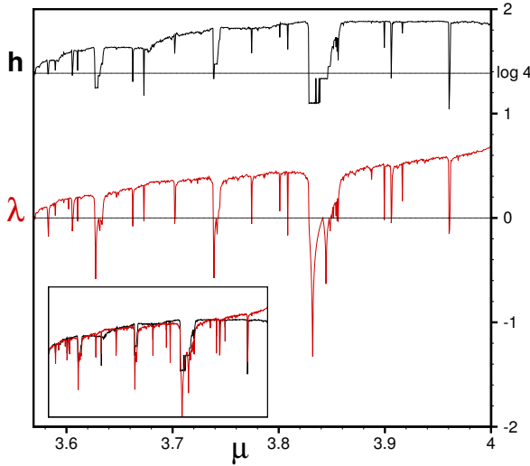
Figure 6 Horizontal visibility network entropy h and Lyapunov exponent \lambda for the Logistic map. We plot the numerical values of h and \lambda for 3.5 < \mu < 4 (the numerical step is \delta\mu = 5 \cdot 10^{-4} and in each case the processed time series have a size of 2^{12} data). The inset reproduces the same data but with a rescaled entropy h - \log(4) . The surprisingly good match between both quantities is due to the Pesin identity (see text). Unexpectedly, the Lyapunov exponent within the periodic windows ( \lambda < 0 inside the chaotic region) is also well captured by h .
