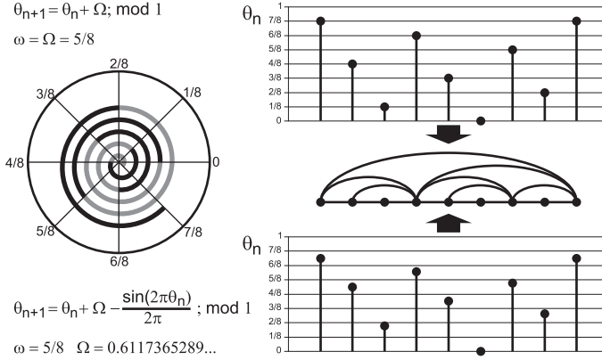
Figure 9 Examples of two standard circle map periodic series with dressed winding number \omega = 5/8 , K = 0 (top) and K = 1 (bottom). As can be observed, the order of visits on the circle and the relative values of \theta_n remain invariant and the associated HV graph is therefore the same in both cases.
