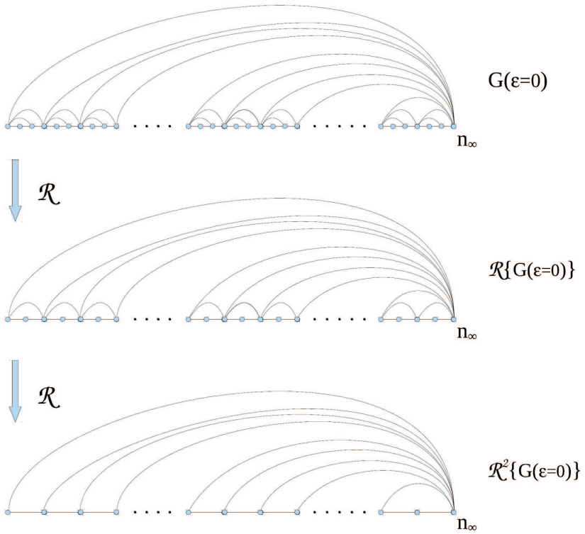
Figure 12 Illustration of the renormalization operator \mathcal{R} applied on the HV graph at \epsilon = 0 . This graph renormalizes, after two iterations of \mathcal{R} , into an HV graph G_c which is itself (i) invariant under \mathcal{R} , and (ii) unstable under perturbations in \epsilon , thus constituting a nontrivial (saddle) fixed point of the graph-theoretical RG flow.
