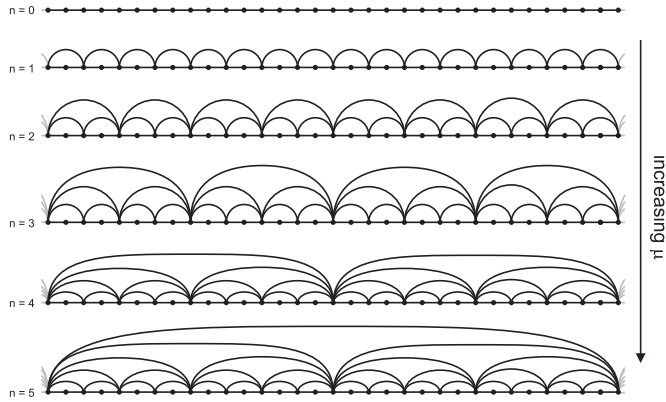
Figure 4 Periodic Feigenbaum graphs for \mu < \mu_\infty . The sequence of graphs associated to periodic attractors with increasing period T = 2^n undergoing a period-doubling cascade. The pattern that occurs for increasing values of the period is related to the universal ordering with which an orbit visits the points of the attractor. Observe that the hierarchical self-similarity of these graphs requires that the graph for n - 1 is a subgraph of that for n .
