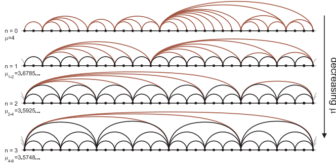
Figure 5 Aperiodic Feigenbaum graphs for \mu > \mu_\infty . A sequence of graphs associated with chaotic series after n chaotic-band reverse bifurcations, starting at \mu = 4 for n = 0 , when the attractor extends along a single band and the degree distribution does not present any regularity (red links). For n > 0 the phase space is partitioned in 2^n disconnected chaotic bands and the n -th self-affine image of \mu = 4 is the n -th Misiurewicz point \mu_{2^n-1-2^n} . In all cases, the orbit visits each chaotic band in the same order as in the periodic region \mu < \mu_\infty . This order of visits induces an ordered structure in the graphs (black links) analogous to that found for the period-doubling cascade.
