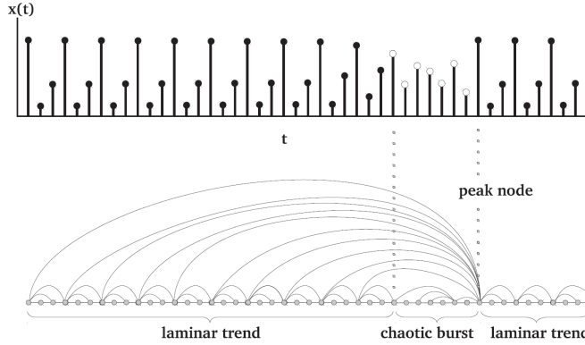
Figure 7 Graphical illustration of how the Horizontal Visibility (HV) graph inherits in its structure the dynamics of the associated intermittent series. In the top of the figure we show a sample intermittent series generated by the logistic map close to \mu_c ( \epsilon > 0 ), producing laminar regions (black) mixed with chaotic bursts (white). In the bottom we plot the associated HV graph. Laminar regions are mapped into nodes with a periodic backbone, whereas the actual pseudoperiodicity of the series is inherited in the graph by the existence of so called peak or interfacial nodes. Chaotic bursts are mapped into chaotic nodes, with a characteristic degree distribution.
