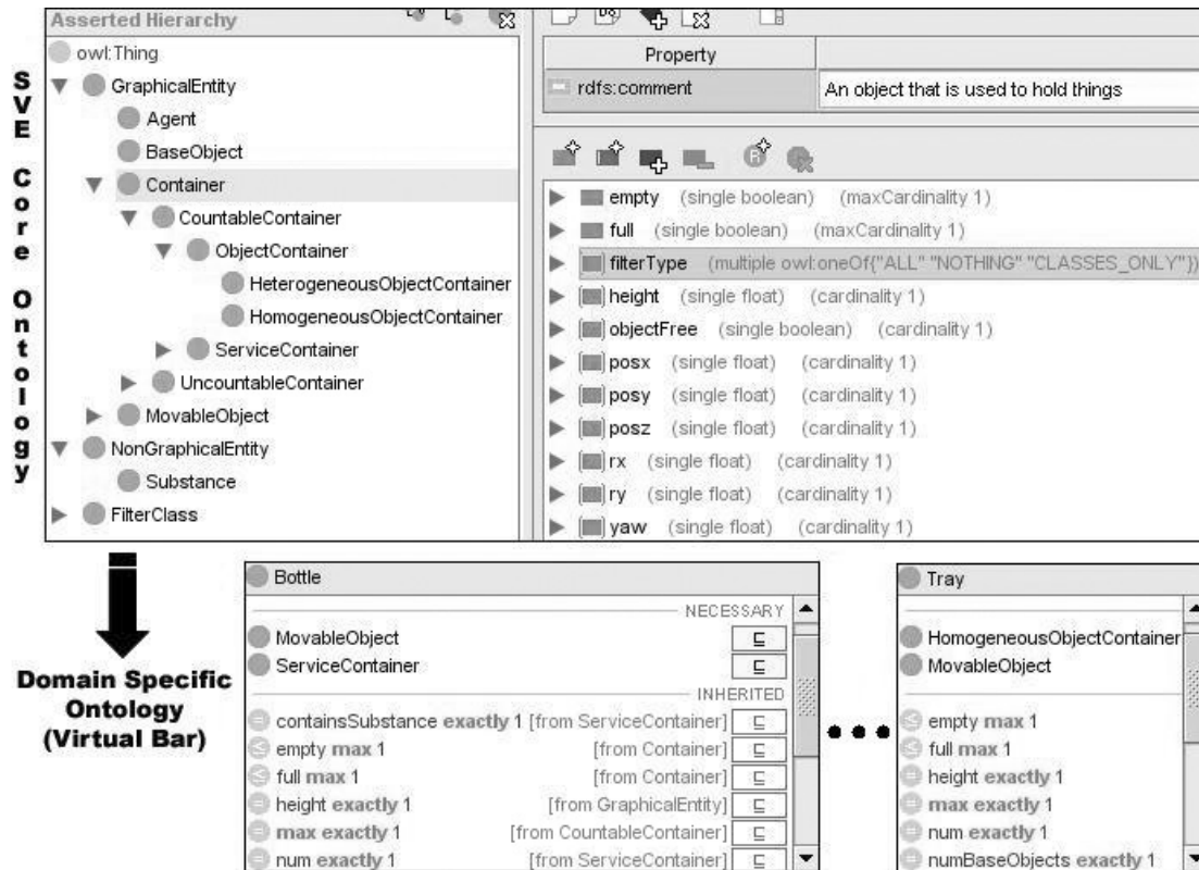
Figure 2 SVE Core Ontology and Virtual Bar Ontology
