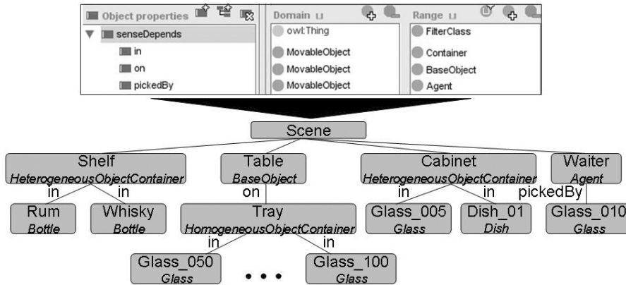
Figure 4 Sensorial dependency tree
