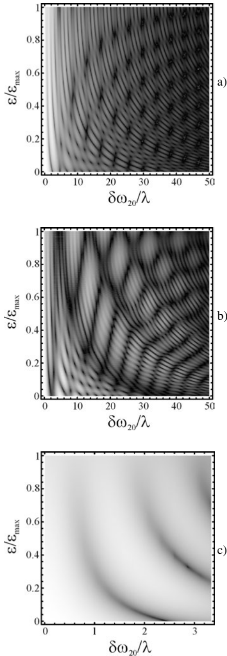
Figure 3. Axial irradiances, in grey levels, given by CRDs constructed with D = 0.5 and N = 4 and with different lacunarity for S = 1 (a) and (c) and S = 2 (b). Note that the scale change in the horizontal axis in (c).
