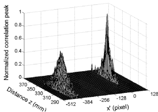
Figure 11. Value of the correlation peak at fixed positions (those of maximum correlation peaks), for input images reconstructed at various propagation distances z .
