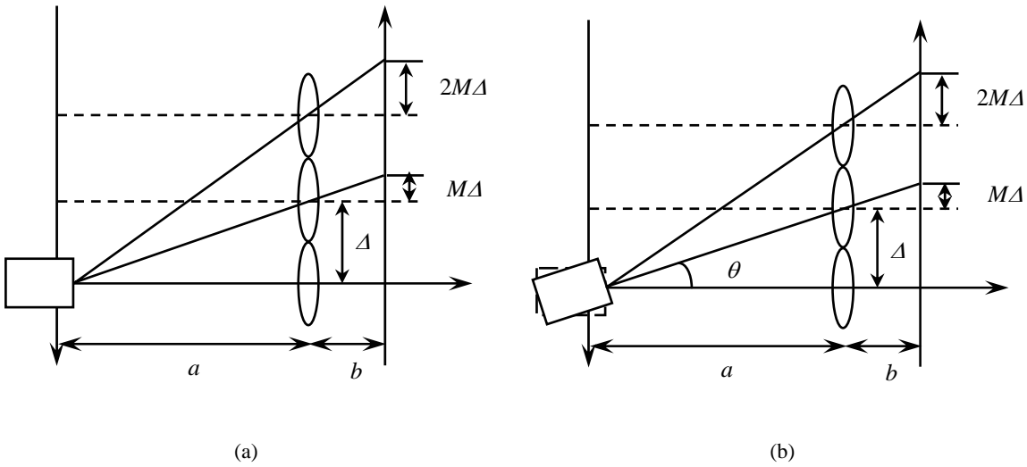
Figure 6. Spatial shift of elemental images when the 3D object is rotated.
