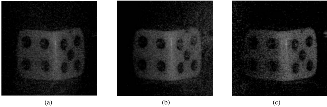
Figure 12. Reconstructed images at 315 mm from the image sensor for three different perspective angles: (a) -0.9^\circ , (b) 0^\circ , and (c) 0.9^\circ .
