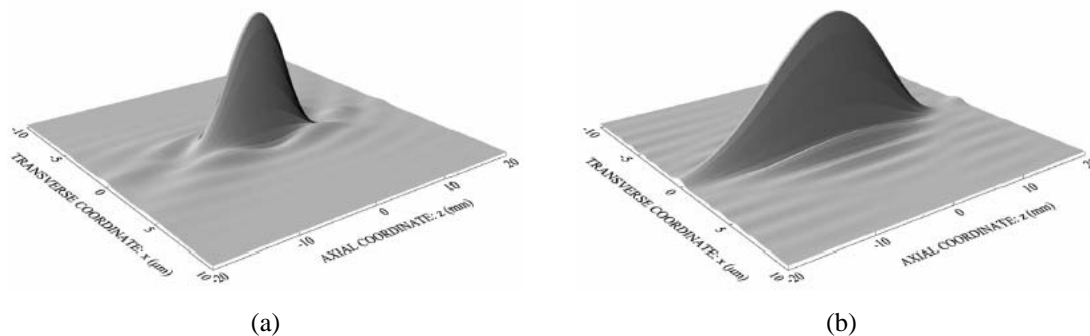
Figure 2. 3D plot of the meridian section of the impulse response for: (a) a conventional microlens and (b) an amplitude-modulated microlens.
