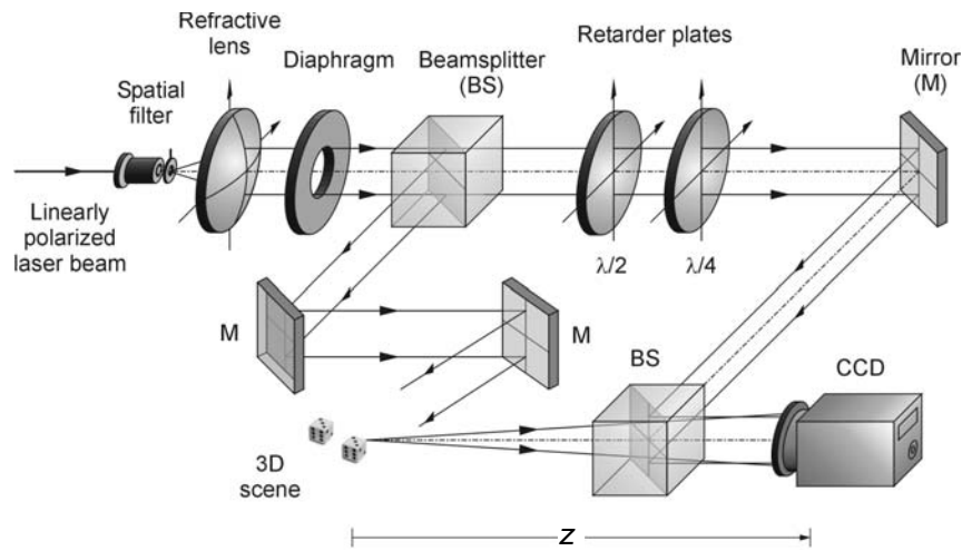
Figure 8. Optical configuration for a four-step phase shifting digital holography system. SP, spatial filter; L, lens; A, aperture; BS's, beamsplitter; M's, mirror; RP's, phase retarder plate.
