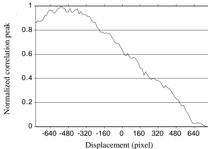
Figure 13. Maximum value of correlation between the reference and the input reconstructed images with different angle of views by use of noncentered windows.
