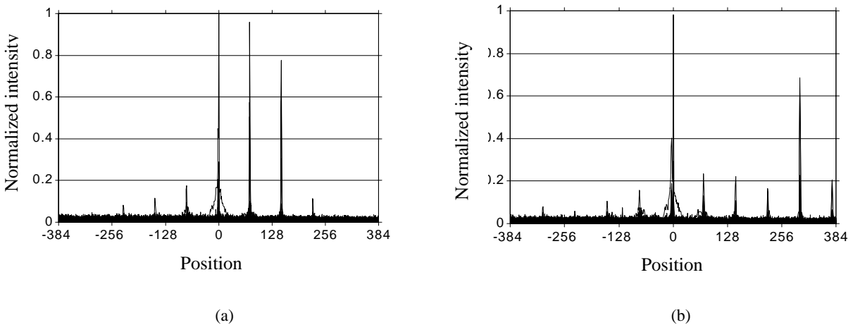
Figure 7. Correlation profile when the die is rotated by an angle of (a) 0.26° and (b) 0.78°.
