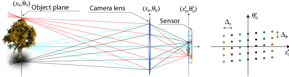
Fig. 1. Scheme of an InI camera and sketch of the sampled radiance map captured with it. The spatial sampling period is \Delta_x = p . The angular sampling period, \Delta_\theta , is the angular size of pixels as seen from the MLA
