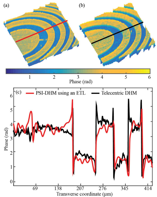
Fig. 4. PSI-DHM versus off-axis telecentric DHM. (a) QPI of a Fresnel's lens by PSI-DHM; (b) QPI of the same Fresnel's lens by off-axis telecentric DHM; and (c) profiles along the lines of panels (a) and (b).
