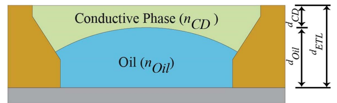
Fig. 2. ETL schematics. In green, the conductive phase with refractive index n_{CD} and in blue, the oil phase with refractive index n_{Oil} . d_{ETL} is the total thickness of the ETL; d_{Oil} , and d_{CD} are thicknesses at the center of the ETL.
