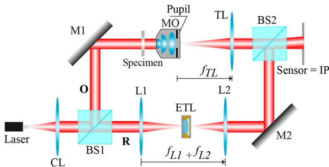
Fig. 1. Proposed set-up to provide PSI using an ETL, which is inserted at the common focal plane of an afocal relay system. CL, collimating lens; BS1 and BS2, cube beam splitters; O, object wave; R, reference wave; M1 and M2, mirrors; L1 and L2, converging lenses. The MO and a TL operated in telecentric configuration.
