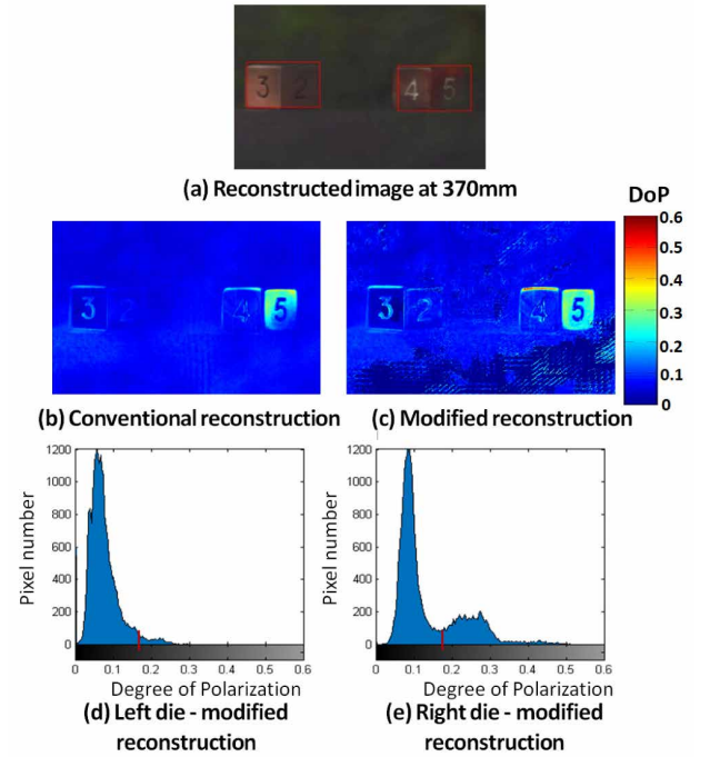
Fig. 27. MOSIS 2.0 for 3-D object shape and material inspection experiments in the presence of occlusion. (a) 3-D reconstructed images at the object planes of 370 mm with target recognition. Degree of polarization reconstructed images at 370 mm (b) by the conventional reconstruction, and (c) by the modified reconstruction method. Distribution of degree of polarization for the target surface reflected lights. (d) Left die by the modified reconstruction in (c), and (e) right die by the modified reconstruction in (c).
