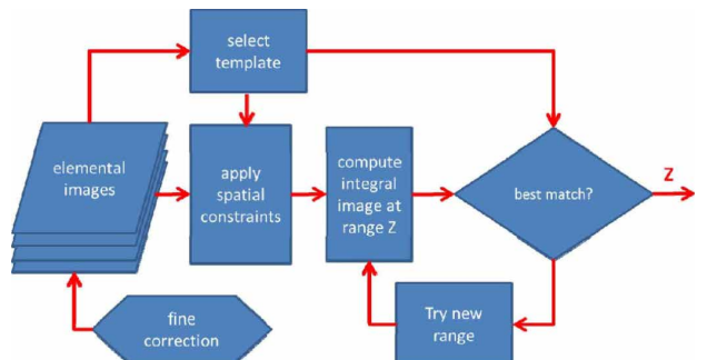
Fig. 14. Overview of the range search algorithm [9].
