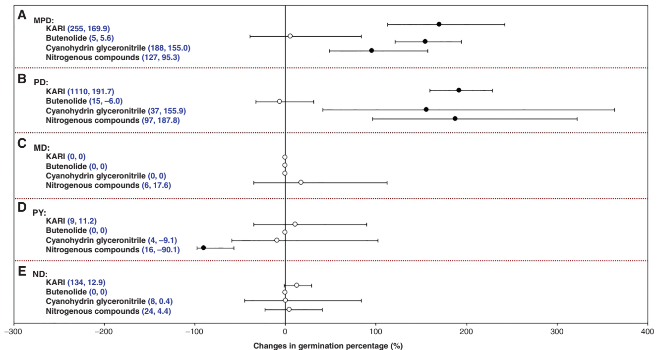
FIG. 4. Relative germination responses of non-dormant (ND) seeds and seeds with different classes of dormancy (MPD, PD, MD, PY) to smoke-derived compounds. Each data point represents the percentage change compared to the control. The first number in parentheses indicates the number of observations and the second represents the mean value. Symbols and bars show the mean response and 95 % confidence interval, respectively. Open circles indicate that estimates are not statistically significantly different from zero at \alpha = 0.05 , while filled symbols indicate significant differences. ND, non-dormant; PD, physiological dormancy; PY, physical dormancy; MD/MPD, morphological dormancy/morphophysiological dormancy.
