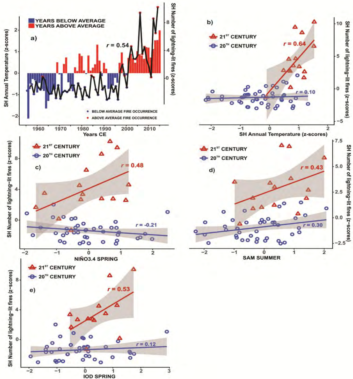
Figure 3 a) Stacked plots of the SH annual temperatures (z-scores; data from ERA-Interim Reanalysis) and the total number of lightning-lit fires recorded in the Southern Hemisphere. b) Scatterplot of the SH annual temperatures (z-scores; data from ERA-Interim Reanalysis) and the total number of lightning-lit fires recorded in the Southern Hemisphere; Black solid line in a) represents the summed SH number of lightning-ignited fires. Colour and symbol coding in b,c,d,e refers to the 20 th (blue dots) and the 21 st (red triangle) centuries. c) Scatterplot of the NIÑO3.4 Index (spring) and the number of lightning-lit fires across the SH; d) Scatterplot of the SAM Index (summer) and the number of lightning-lit fires across the SH; e) Scatterplot of the IOD Index (spring) and the number of lightning-lit fires across the SH.
