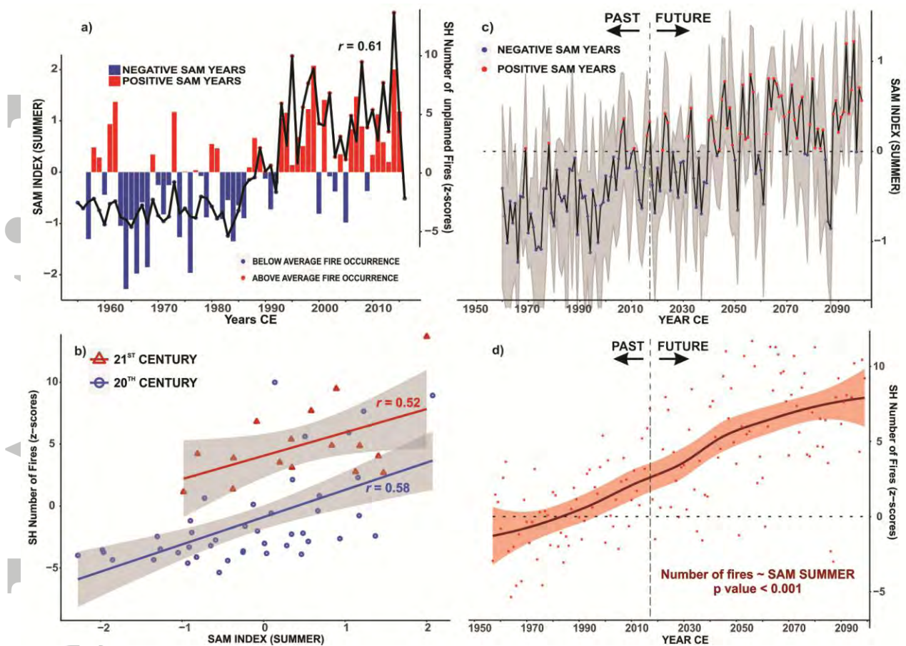
Figure 2 a) Stacked plots of the SAM Index (summer) and the total number of wildfires in the Southern Hemisphere (black solid line; only regions with a positive correlation with the SAM Index are included in the summed record) from all ignition sources and vegetation types combined; b) Scatterplot of the two time-series shown in a). Colour and symbol coding refers to the 20 th (blue dots) and the 21 st (red triangle) centuries; c) Summer SAM Index projection under increasing greenhouse gases concentrations (data from Thompson et al., 2011 and McLandress et al. , 2011); d) Linear model projecting the total (human and lightning-lit) wildfire occurrences in the SH extending to the year 2100 based on the SAM Index projection presented in c). Pearson correlation coefficients are reported in a) and b).
