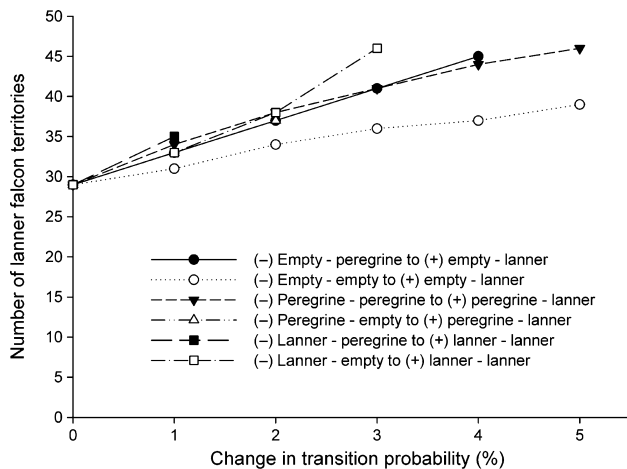
Figure 3 Results of elasticity analysis of the transition matrix of the baseline scenario. The figure shows lanner falcon final population size in Sicily under different scenarios. Increasing the probability of lanner falcon: (1) colonizing empty territories (empty–lanner), (2) replacing territories occupied by peregrines (peregrine–lanner) and (3) persistence of territories (lanner–lanner). Changes in transitions are similar to those in Fig. 2. Symbols (+) and (–) indicate increase or decrease in the corresponding transition probability.
