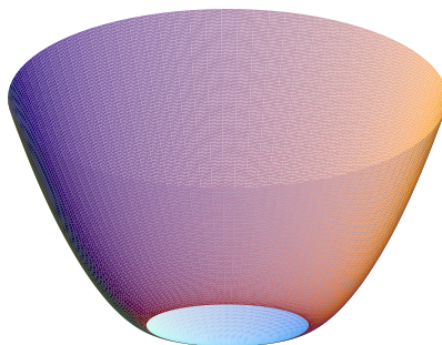
Figure 1. Plot of a piece of the unique revolution surface with nongeodesic biharmonic parallel lines, for c = 1 and c_1 = 0 .
