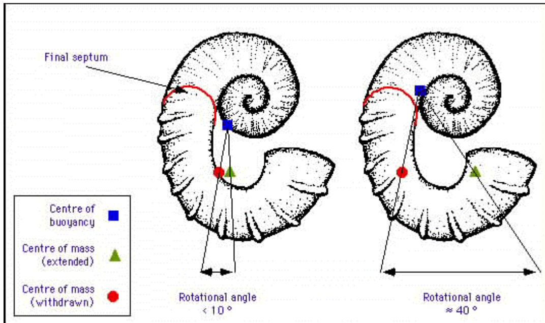
Figure 1. Centres of buoyancy (blue squares) and mass (green triangle and red circle) for Tropaeum hillsi deduced using Trueman's model with the body chamber entirely filled (left); and the model presented herein, with the body chamber only partially filled (right). The green triangle indicates the position of the centre of mass when the head and arms are extended; the red circles when withdrawn.
