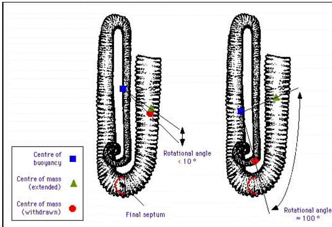
Figure 3. Centres of buoyancy (blue squares) and mass (green triangle and red circle) for Hamites maximus deduced using Trueman's model with the body chamber entirely filled (left); and the model presented here, with the body chamber only partially filled (right). The green triangle indicates the position of the centre of mass when the head and arms are extended; the red circles when withdrawn.
