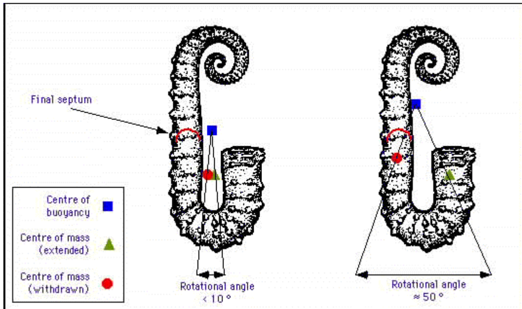
Figure 2. Centres of buoyancy (blue squares) and mass (green triangle and red circle) for Ancycloceras matheronianum deduced using Trueman's model with the body chamber entirely filled (left); and the model presented here, with the body chamber only partially filled (right). The green triangle indicates the position of the centre of mass when the head and arms are extended; the red circles when withdrawn.
