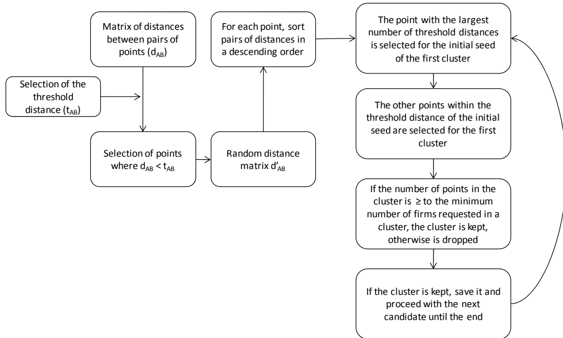
Figure 2. Spatial nearest neighbour hierarchical clustering algorithm
