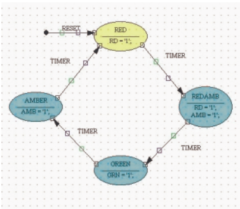
FIGURE 4-19: STATE DIAGRAM
