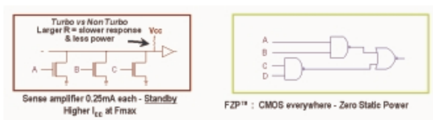
FIGURE 2-21: SENSE AMPLIFIER VS. CMOS CPLDS
