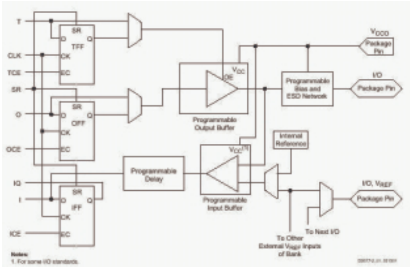
FIGURE 2-10: SPARTAN-III INPUT/OUTPUT BLOCK
