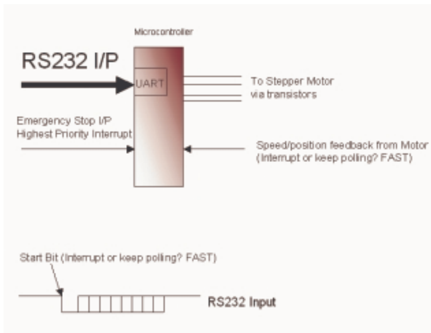
FIGURE 7-6: MICROCONTROLLER IMPLEMENTATION
