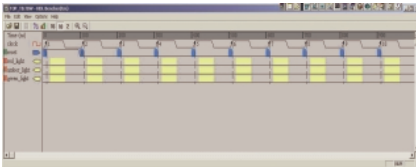
FIGURE 4-38: Waveform Diagram
