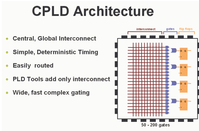
FIGURE 1-3: CPLD ARCHITECTURE
