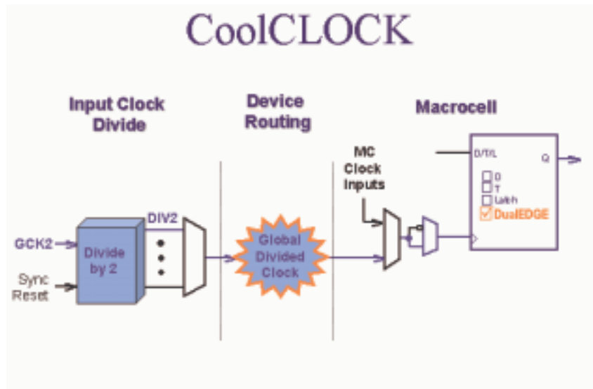
FIGURE 2-36: COOLCLOCK
