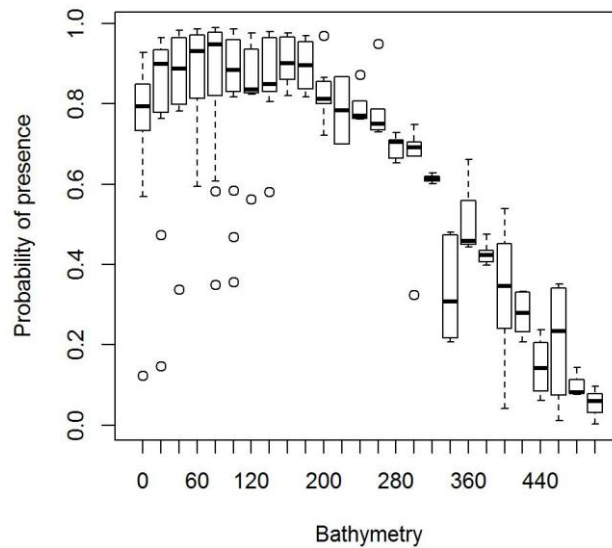
Figure 4: Boxplot of the mean of the fitted values at the prediction nodes of the occurrence model. Each boxplot corresponds to a 20 meter interval.
