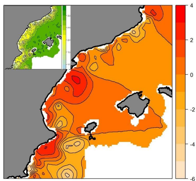
Figure 3: The posterior mean and standard deviation (top-left) of the spatial effect in the occurrence model. Pale contours correspond to low values, whilst dark contours indicate high increments in the linear predictor and high standard deviations.
