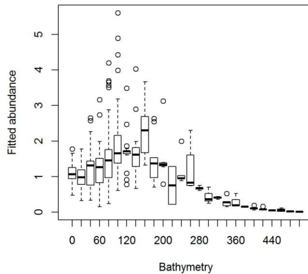
Figure 8: Boxplot of the mean of the fitted values at the prediction nodes of the abundance model. Each boxplot corresponds to a 20 meter interval.
