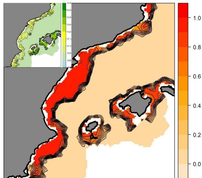
Figure 2: Merluccius merluccius recruits. Spatio-temporal occurrence model output maps in the Western Mediterranean. Average posterior mean estimates of the probability of presence and its standard deviation (top-left) during the study time window. Pale contours correspond to low values, whilst dark contours indicate high probability estimates and standard deviations.
