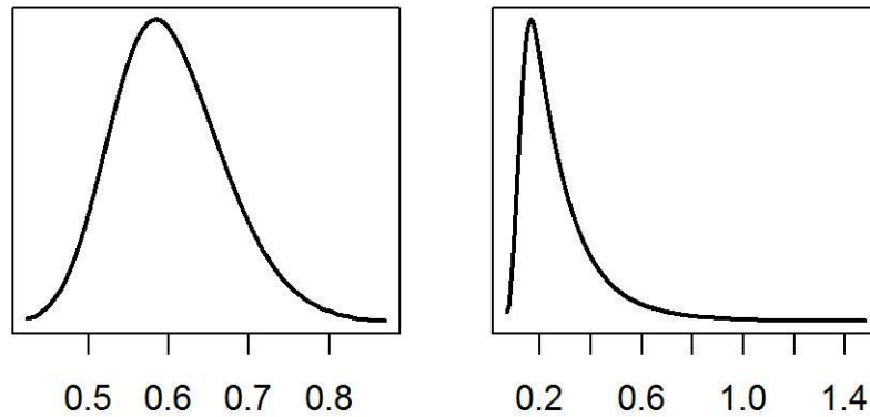
Figure 9: Estimated variance of the spatial effect (left) and estimated variance of the independent random effect for year (right) in the abundance model.
