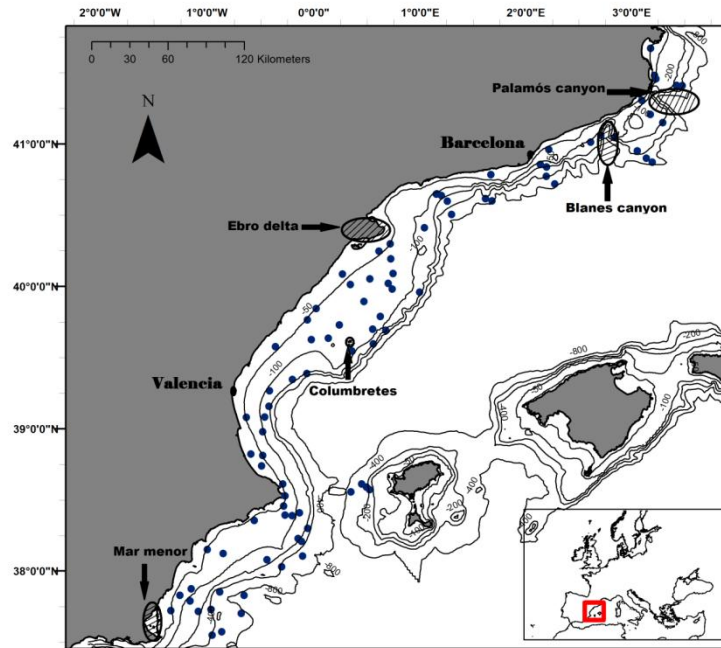
Figure 1: Study area and expected distribution of the samples each year. Bathymetric contours are shown up to the 800 m depth strata according to the MEDITS sampling range.
