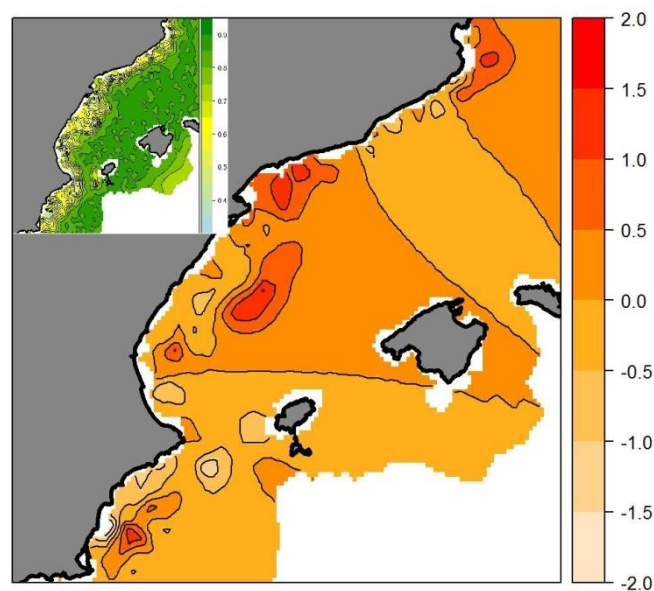
Figure 6: Merluccius merluccius recruits. Spatio-temporal abundance model output maps in the Western Mediterranean. Average posterior mean abundance estimates in kg per 30 minute tow using MEDITS gear and its standard deviation (top-left) during the study time window. Pale contours correspond to low values, whilst dark contours indicate high abundance estimated and standard deviations.
