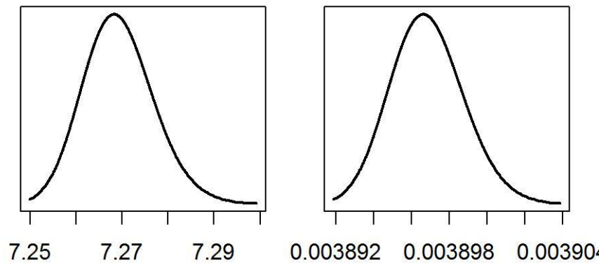
Figure 5: Estimated variance of the spatial effect (left) and estimated variance of the independent random effect for year (right) in the occurrence model. Note the different scale in which the variance is measured.
