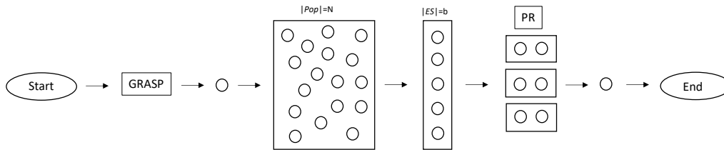
Figure 2: Static GRASP with PR.
