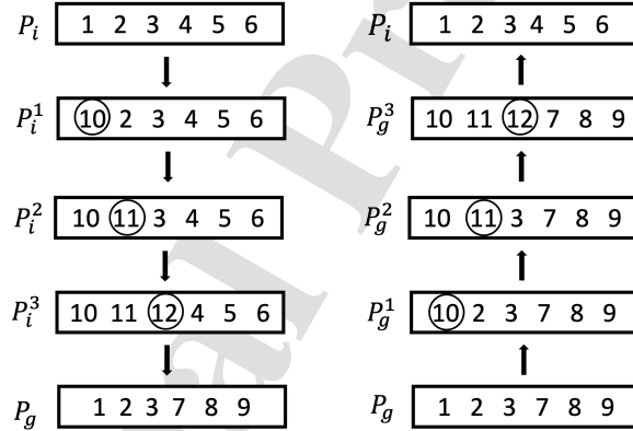
Figure 6: Exterior Path Relinking.
