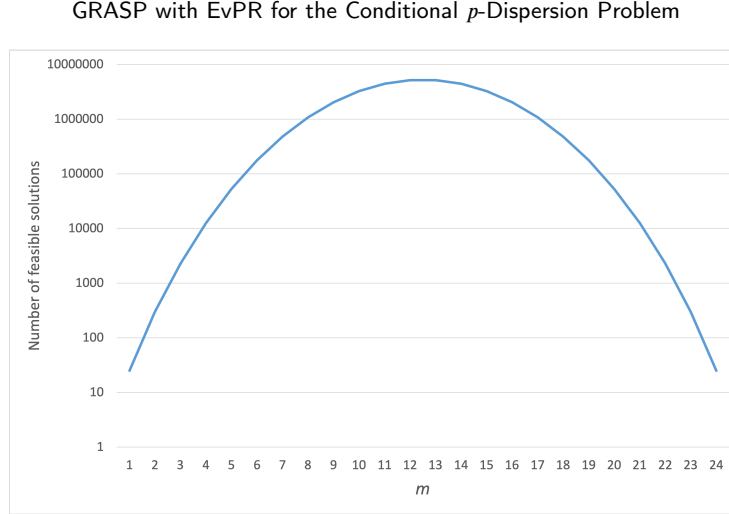
Figure 1: Number of solutions, as a function of m = p + q in the x -axis, of an instance with n = 25 .
