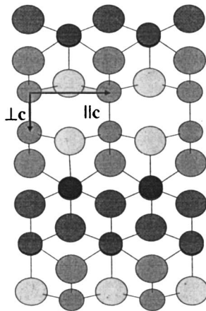
FIG. 1. (a) GaTe structure. (b) GaTe layer top view. In both drawings, the crystallographic c axis and its perpendicular (in the plane of the layer) are drawn. Nonequivalent atoms have different shadowing. Big and small circles correspond to Te and Ga atoms, respectively. View (b) corresponds to the plane of polarization of the x rays.
