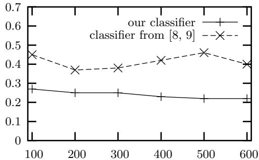
Fig. 2. Size of learning set versus error. Test set constant size 1,000 photos and 1,000 cartoons.
